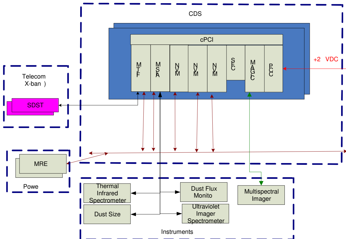
Figure 8: Block Diagram of the CDS System
