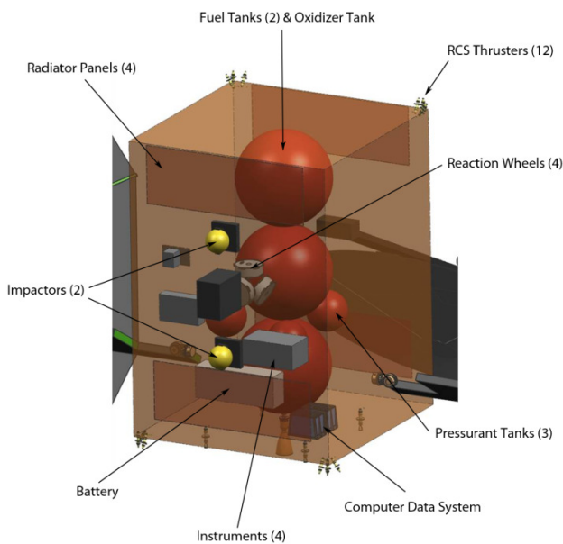
Figure 4: Internal Structure of SHOTPUT
