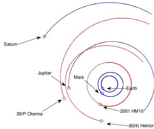
Figure 1: A view of the solar system including the location of the small-bodies of interest at the time of the Oterma encounter.
