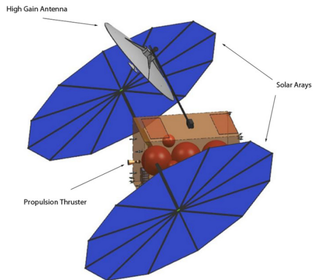
Figure 3: External Structure of SHOTPUT
