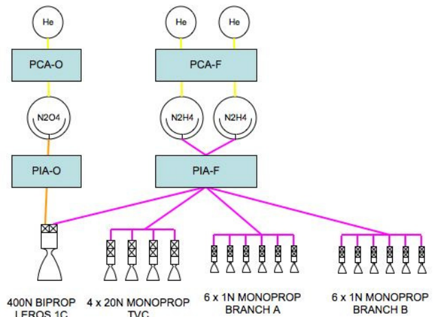
Figure 6: RCS and TVC Thruster Architecture
